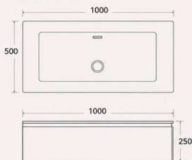
WASHBASIN (mm)
